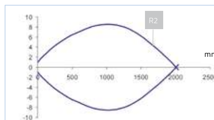
Coaxial polarized retroreflex for transparents (S8...T50/T53)
